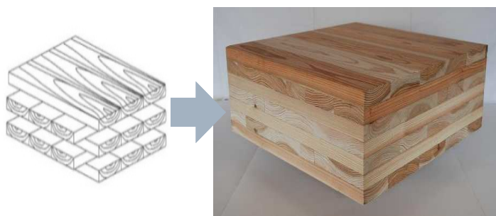
CLT(Cross Laminated Timber)
